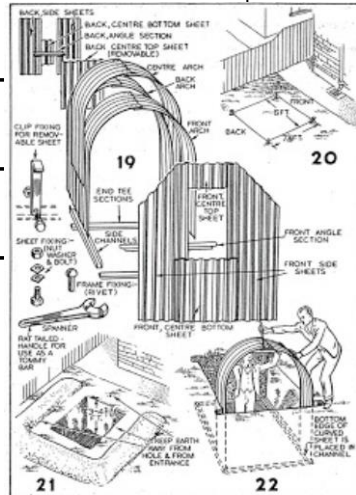
19. The individual parts of the Government Steel Shelter as they are delivered, with detail of each part. 20. The actual size shown should first be marked out in the ground. 21. The diagram shows the hole dug to its final depth. 22. Erecting the end section. Two men are required for this part of the task.
