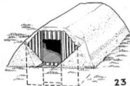
23. The Government Steel Shelter actually in position and provided with an earth covering. A hole is dug in front of the shelter to a depth of 18 inches, and it is recommended that a minimum of 18 inches of soil be provided.
